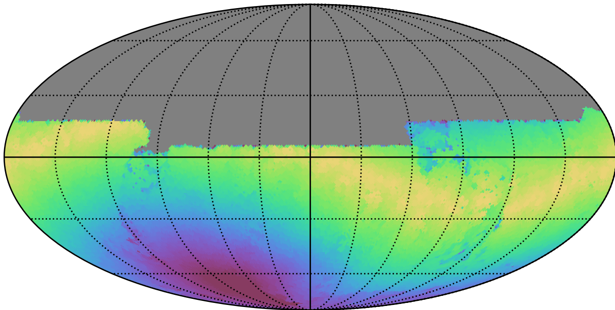
weather_cloudso1v3.4_10yrs All sky u band: Max moonDistance
