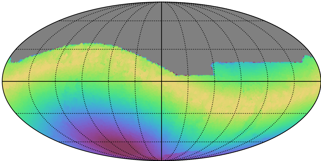
weather_cloudso1v3.4_10yrs All sky r band: Max moonDistance
