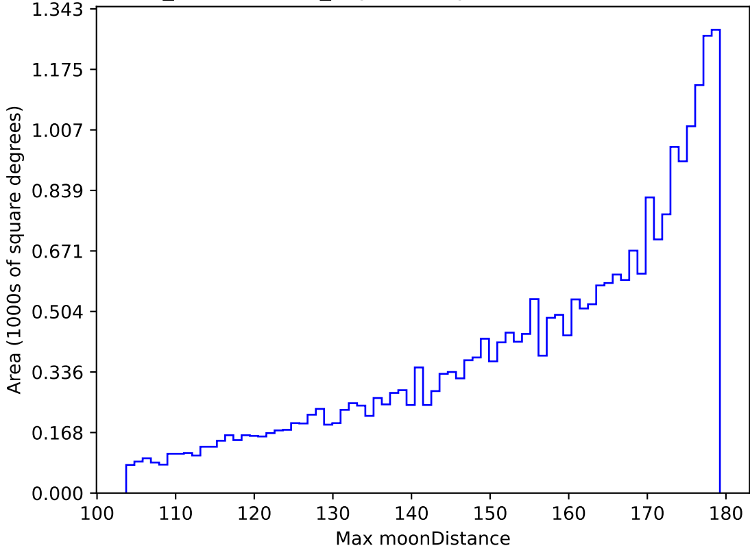
weather_cloudso1v3.4_10yrs All sky r band: Max moonDistance
