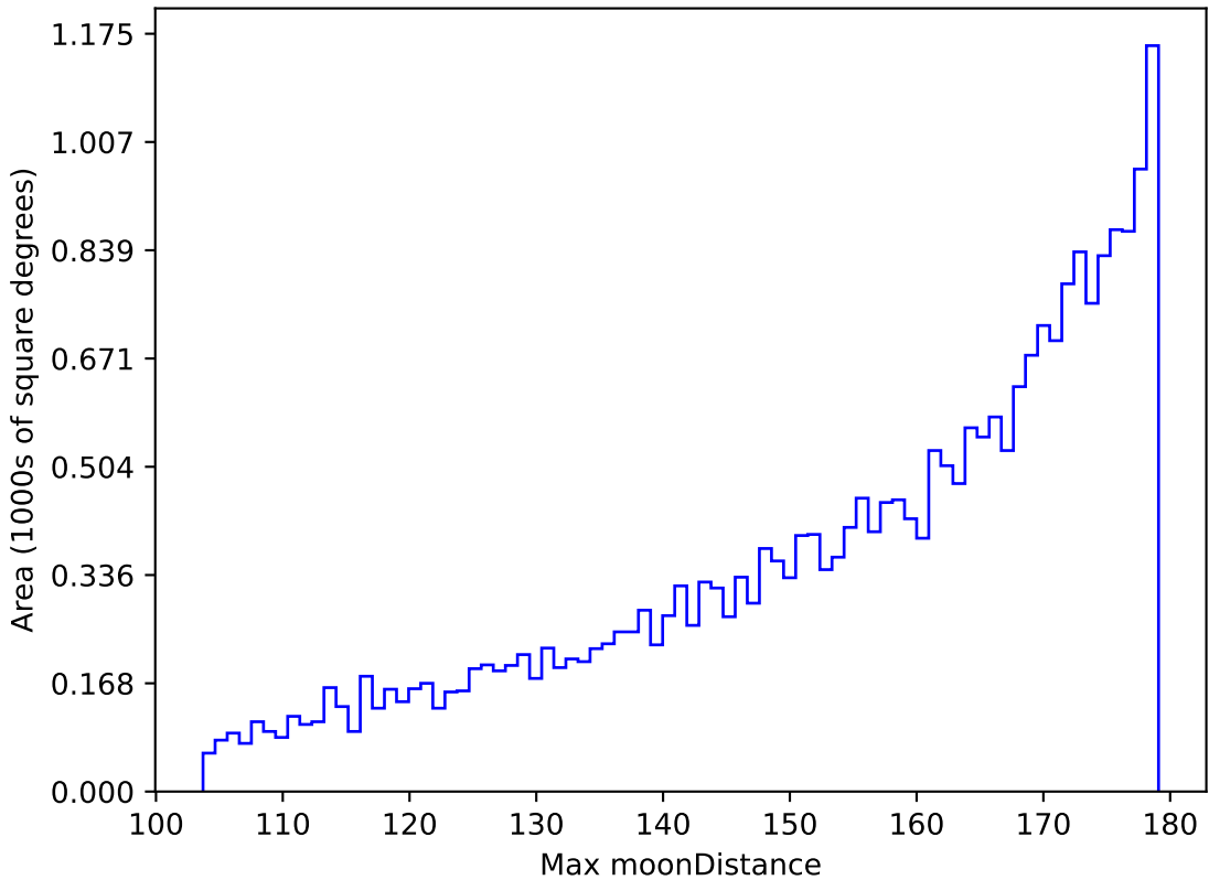
weather_cloudso1v3.4_10yrs All sky i band: Max moonDistance
