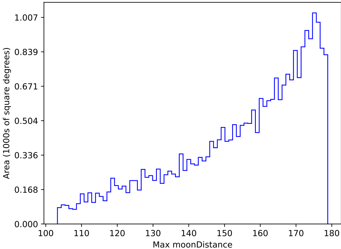
weather_cloudso1v3.4_10yrs All sky g band: Max moonDistance
