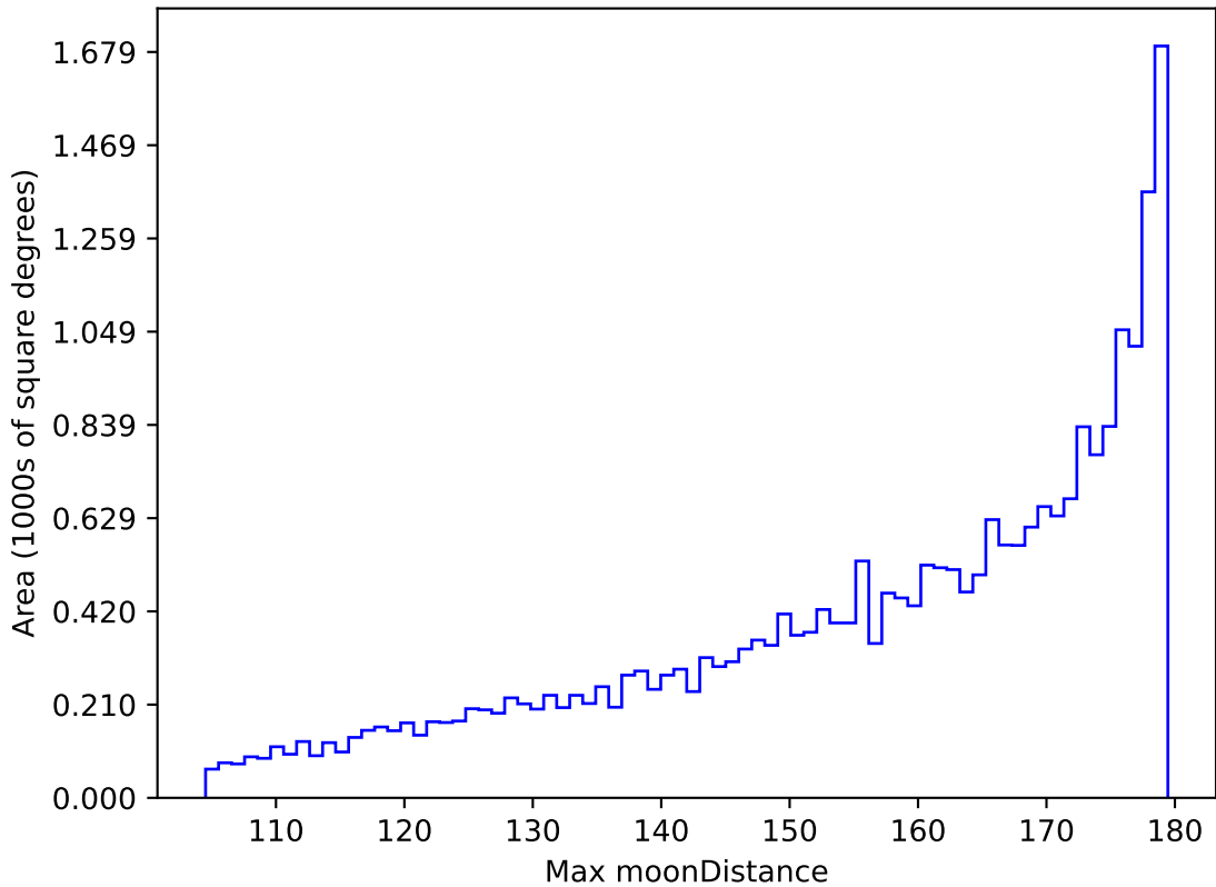
weather_cloudso1v3.4_10yrs All sky all bands: Max moonDistance
