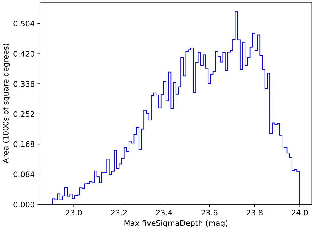
weather_cloudso1v3.4_10yrs Yr 1 u band: Max fiveSigmaDepth
