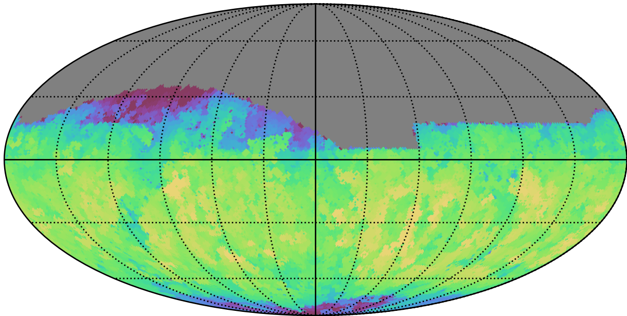
weather_cloudso1v3.4_10yrs Yr 1 i band: Max fiveSigmaDepth
