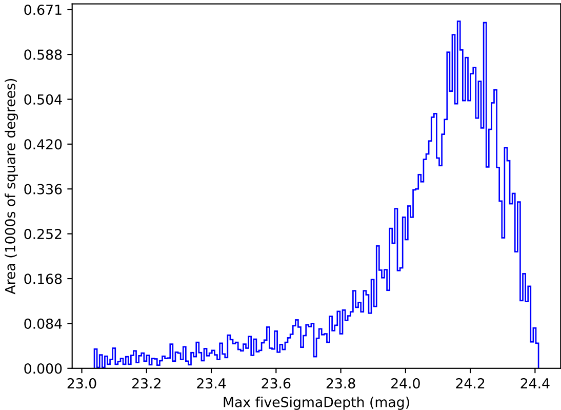
weather_cloudso1v3.4_10yrs Yr 1 i band: Max fiveSigmaDepth
