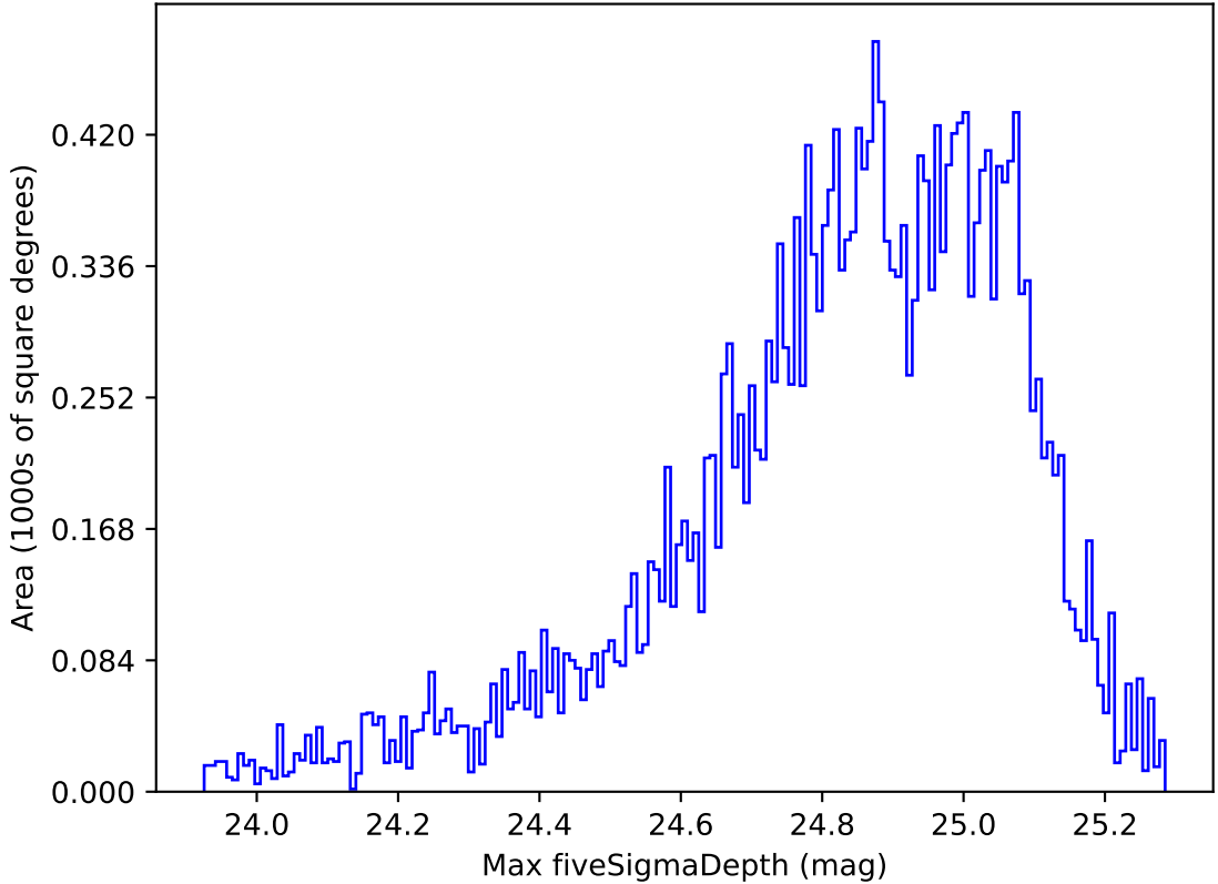
weather_cloudso1v3.4_10yrs Yr 1 g band: Max fiveSigmaDepth
