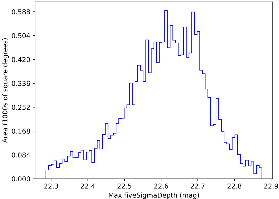
weather_cloudso1v3.4_10yrs WFD y band: Max fiveSigmaDepth
