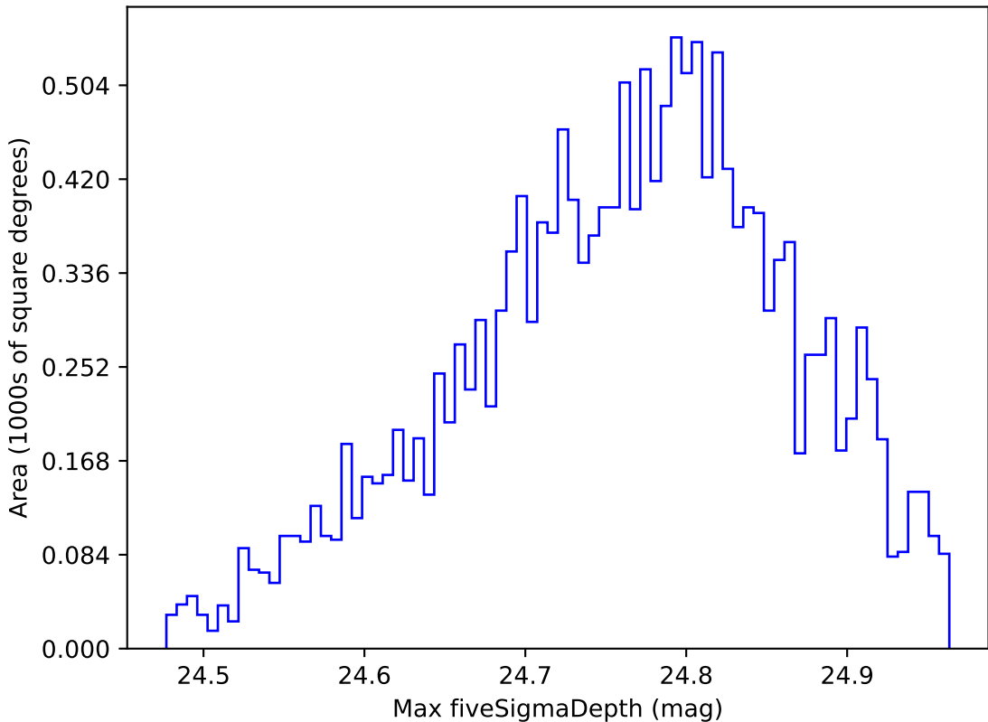
weather_cloudso1v3.4_10yrs WFD r band: Max fiveSigmaDepth
