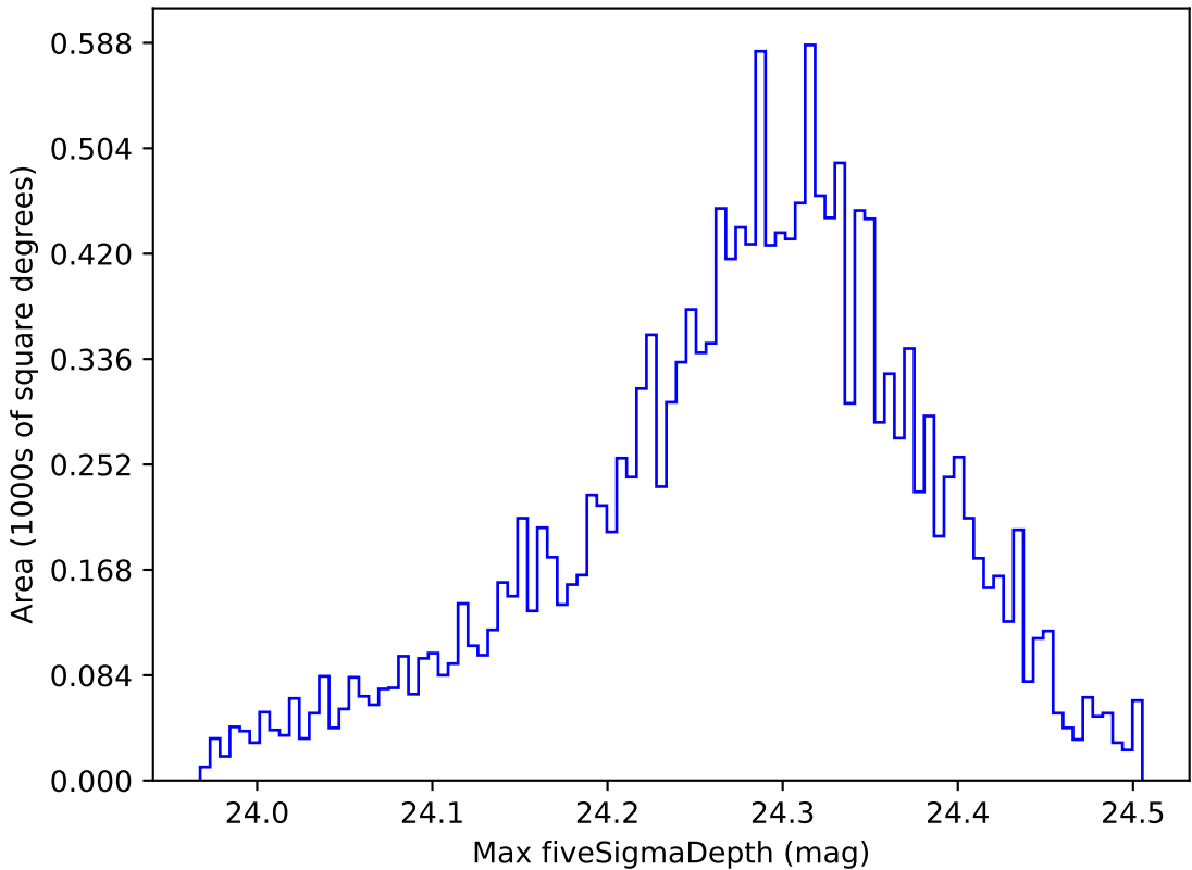
weather_cloudso1v3.4_10yrs WFD i band: Max fiveSigmaDepth
