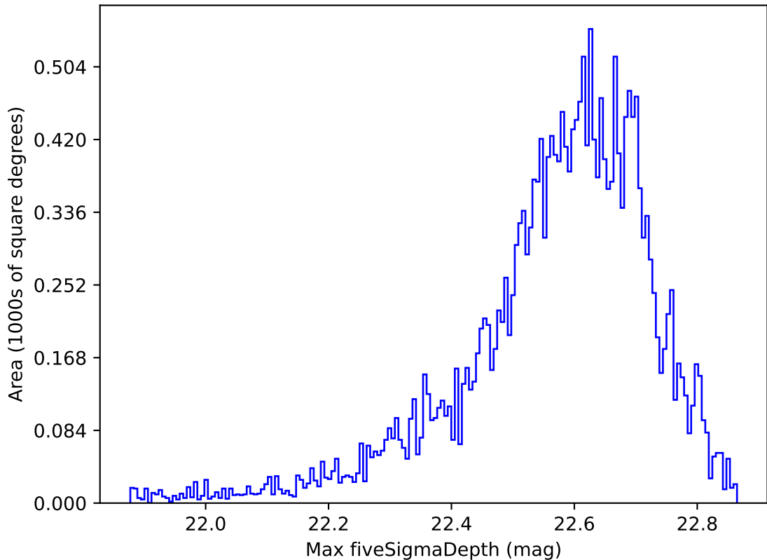
weather_cloudso1v3.4_10yrs All sky y band: Max fiveSigmaDepth
