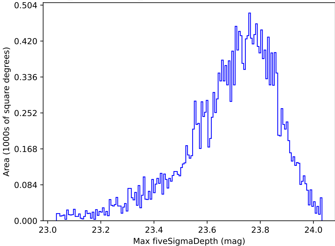
weather_cloudso1v3.4_10yrs All sky u band: Max fiveSigmaDepth
