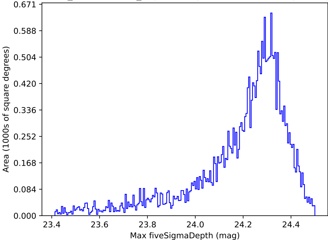
weather_cloudso1v3.4_10yrs All sky i band: Max fiveSigmaDepth
