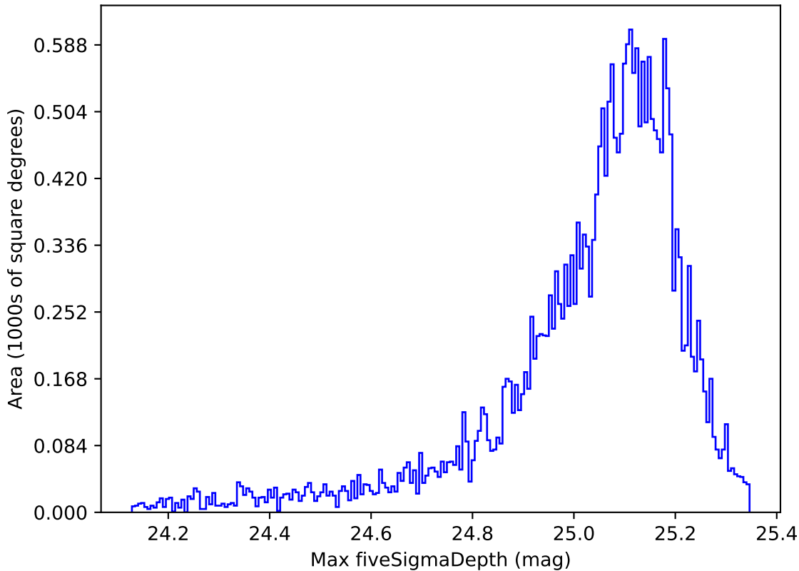
weather_cloudso1v3.4_10yrs All sky all bands: Max fiveSigmaDepth
