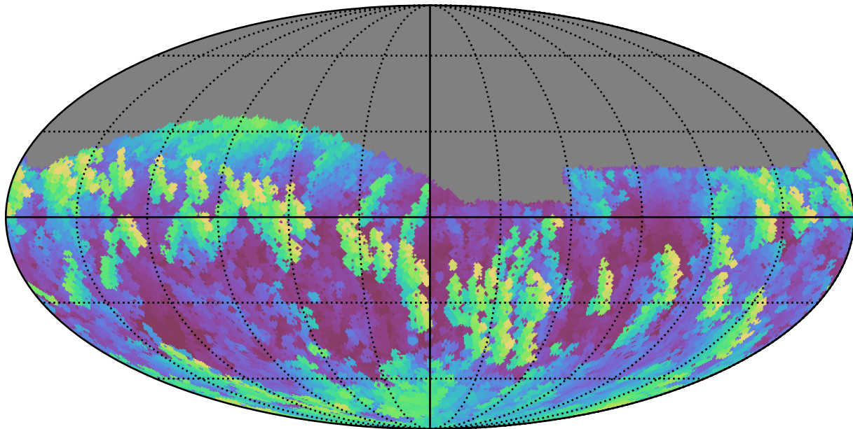
weather_cloudso1v3.4_10yrs Yr 1 z band: Max airmass
