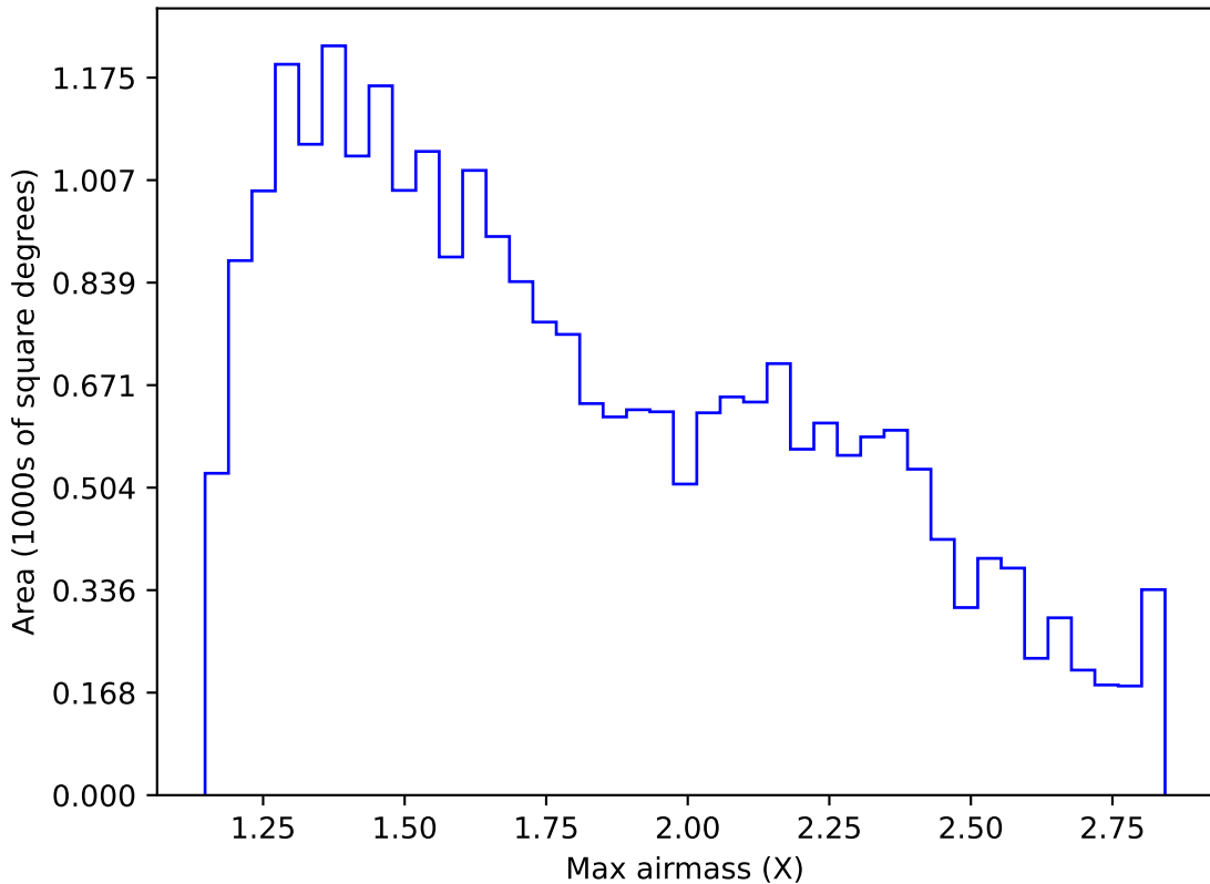
weather_cloudso1v3.4_10yrs Yr 1 z band: Max airmass
