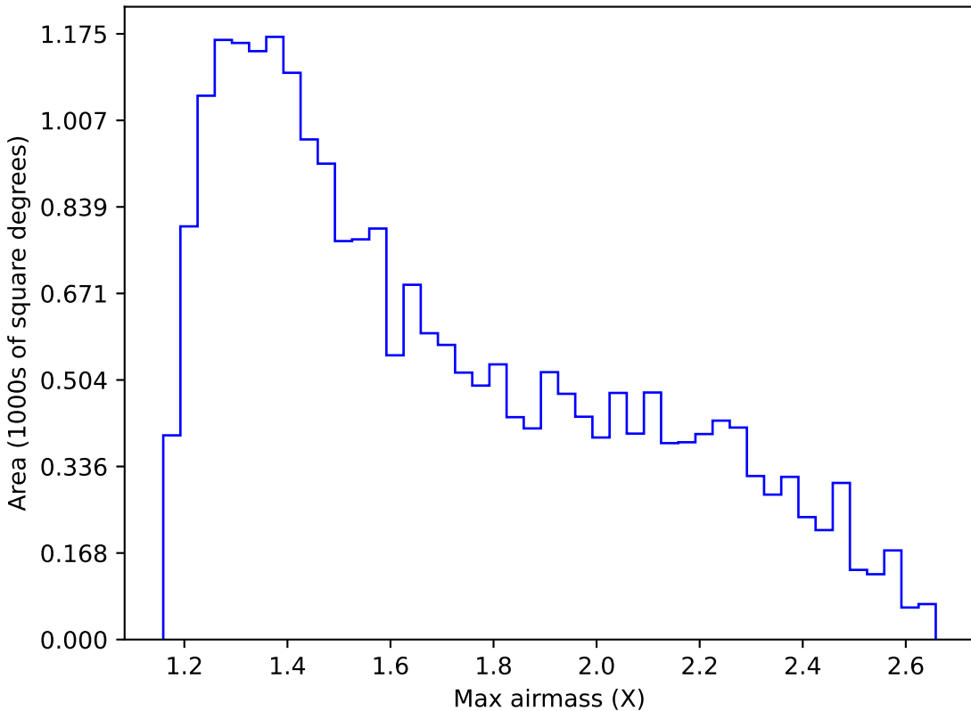
weather_cloudso1v3.4_10yrs Yr 1 y band: Max airmass
