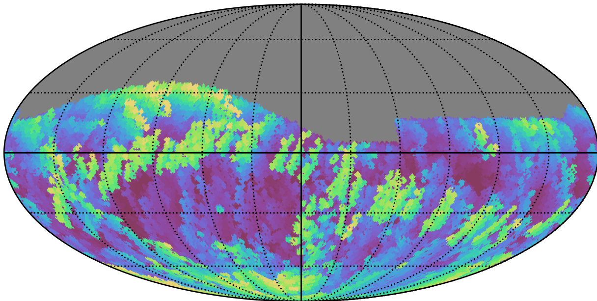
weather_cloudso1v3.4_10yrs Yr 1 r band: Max airmass
