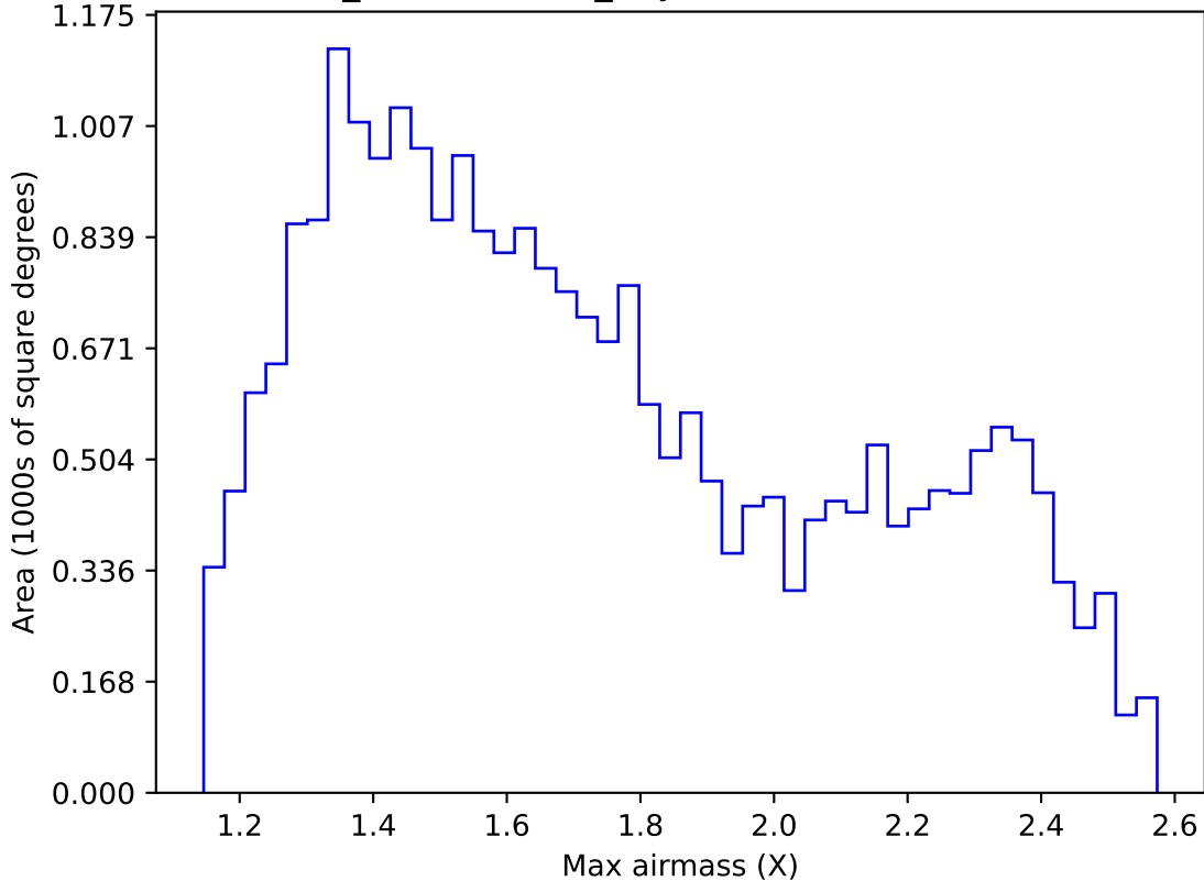
weather_cloudso1v3.4_10yrs Yr 1 r band: Max airmass
