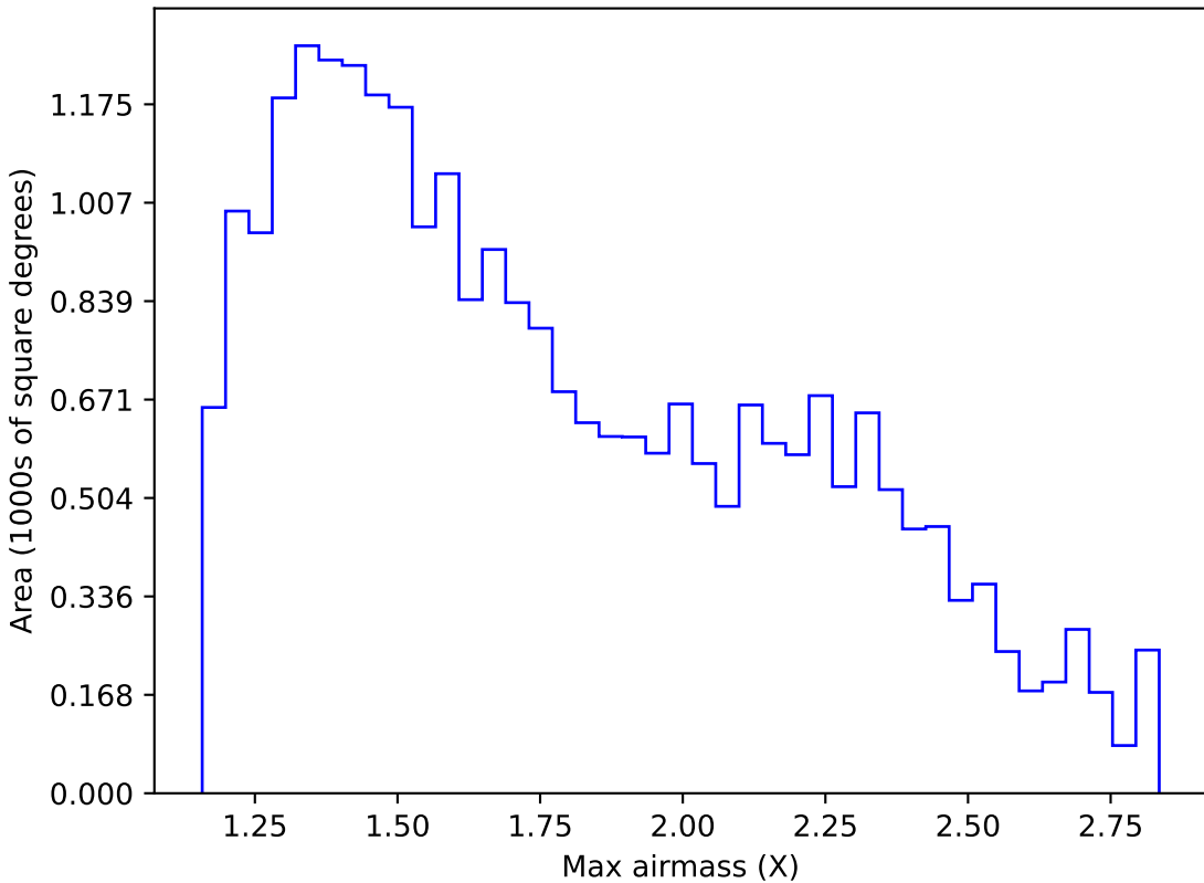
weather_cloudso1v3.4_10yrs Yr 1 i band: Max airmass
