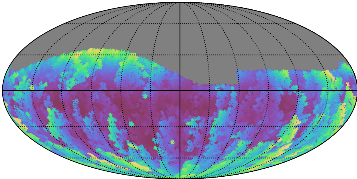
weather_cloudso1v3.4_10yrs Yr 1 g band: Max airmass
