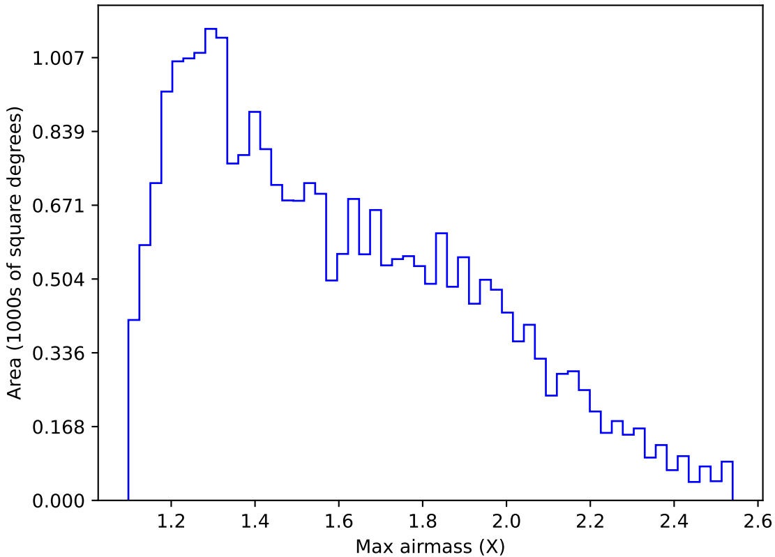
weather_cloudso1v3.4_10yrs Yr 1 g band: Max airmass
