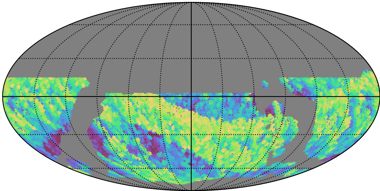
weather_cloudso1v3.4_10yrs WFD z band: Max airmass
