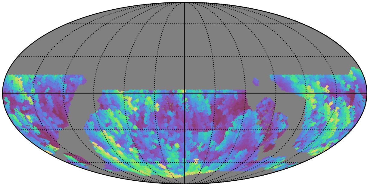
weather_cloudso1v3.4_10yrs WFD u band: Max airmass
