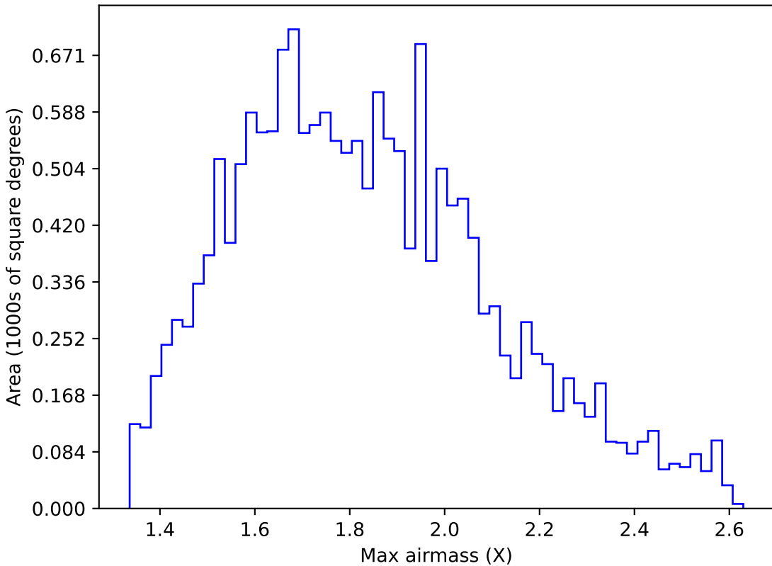
weather_cloudso1v3.4_10yrs WFD u band: Max airmass
