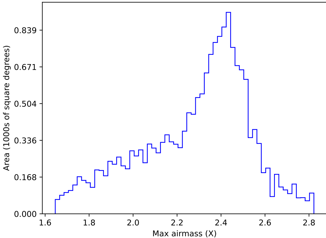
weather_cloudso1v3.4_10yrs WFD r band: Max airmass
