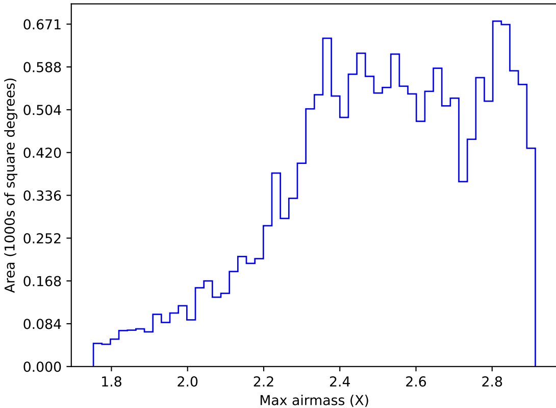
weather_cloudso1v3.4_10yrs WFD i band: Max airmass
