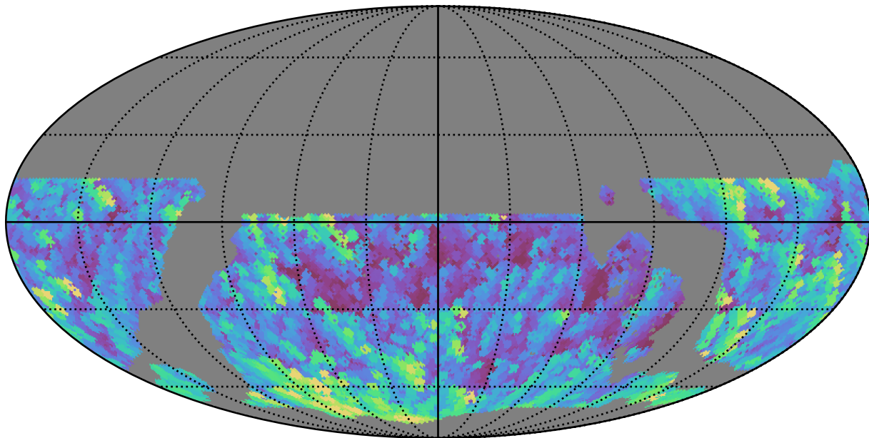
weather_cloudso1v3.4_10yrs WFD g band: Max airmass
