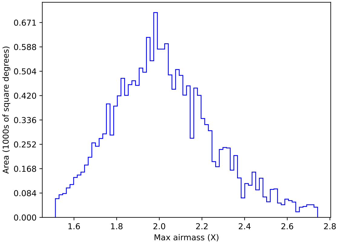
weather_cloudso1v3.4_10yrs WFD g band: Max airmass
