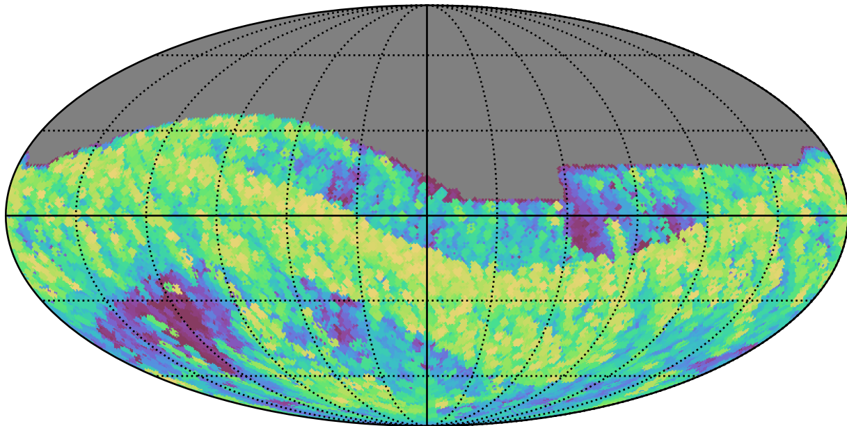
weather_cloudso1v3.4_10yrs All sky z band: Max airmass
