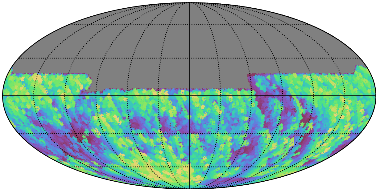
weather_cloudso1v3.4_10yrs All sky y band: Max airmass
