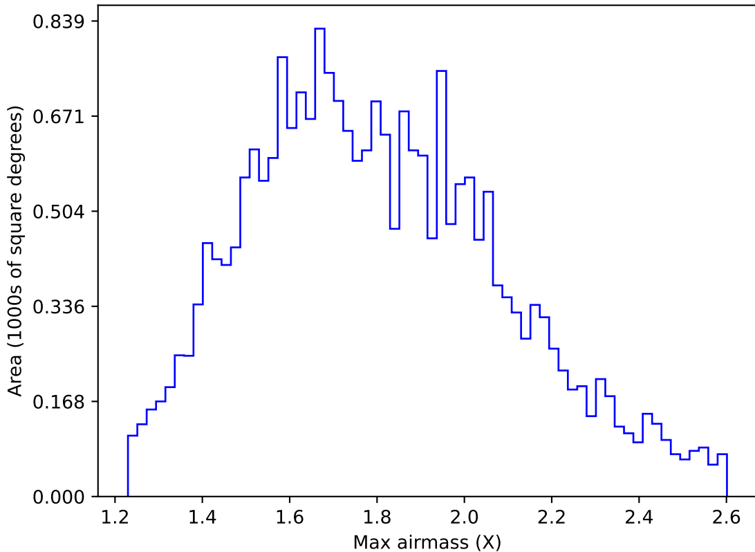
weather_cloudso1v3.4_10yrs All sky u band: Max airmass
