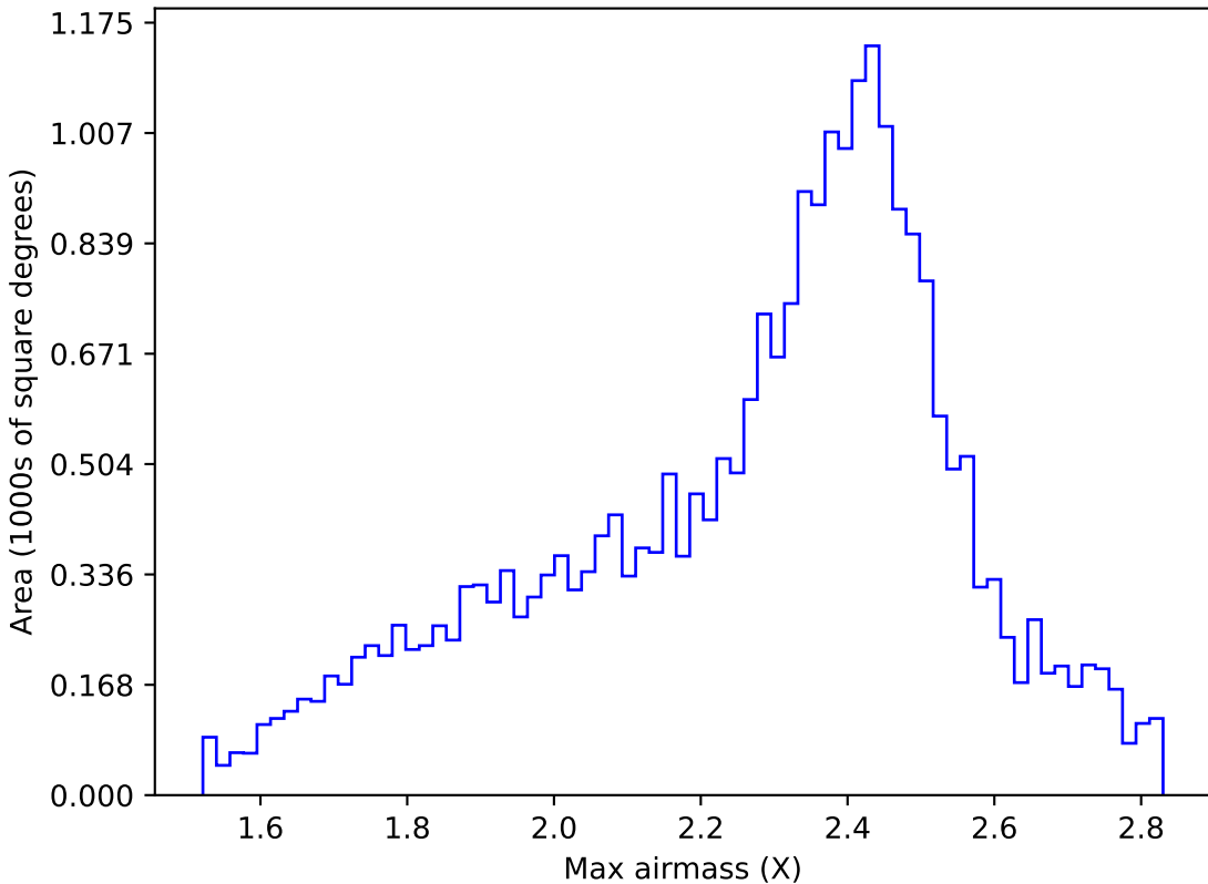
weather_cloudso1v3.4_10yrs All sky r band: Max airmass
