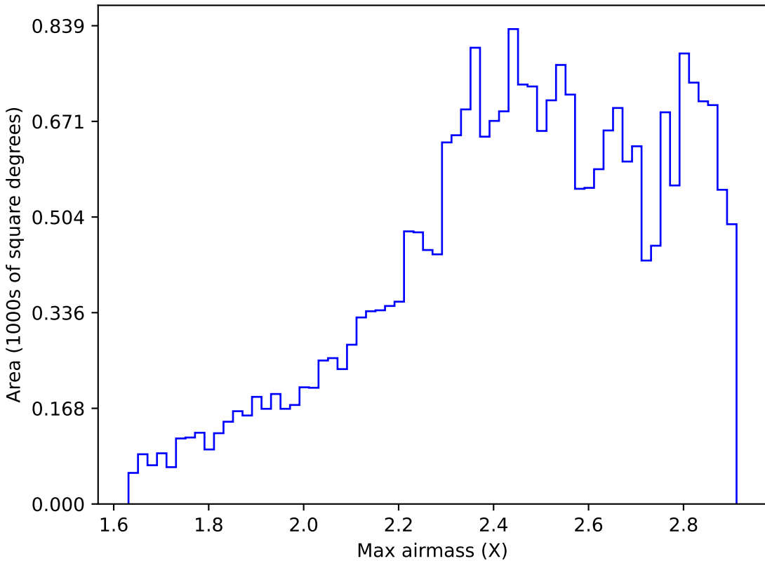
weather_cloudso1v3.4_10yrs All sky i band: Max airmass
