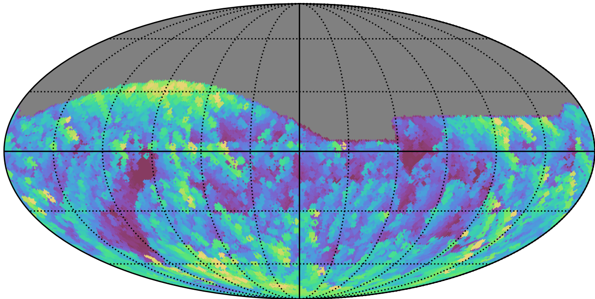
weather_cloudso1v3.4_10yrs All sky g band: Max airmass
