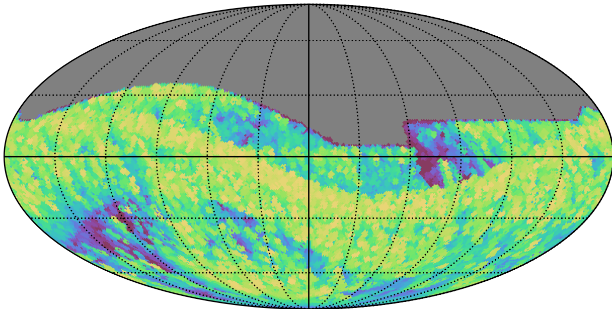
weather_cloudso1v3.4_10yrs All sky all bands: Max airmass
