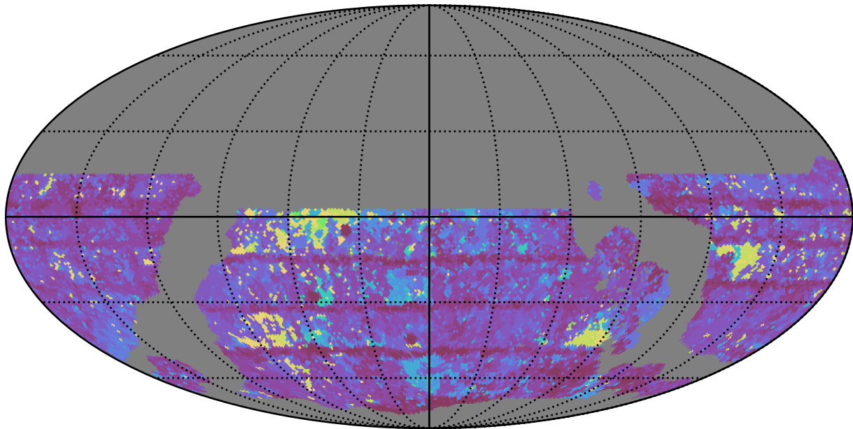
weather_cloudso1v3.4_10yrs WFD y band: Max Inter-Night Gap
