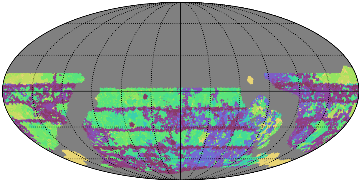
weather_cloudso1v3.4_10yrs WFD u band: Max Inter-Night Gap
