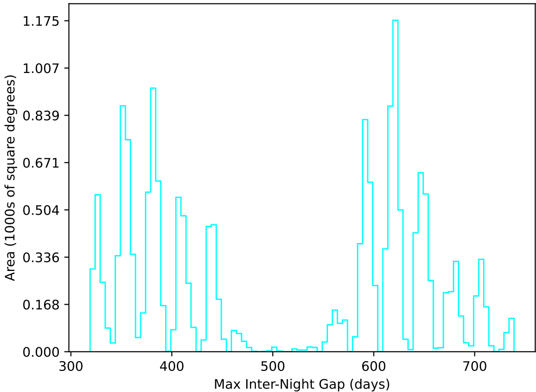
weather_cloudso1v3.4_10yrs WFD u band: Max Inter-Night Gap
