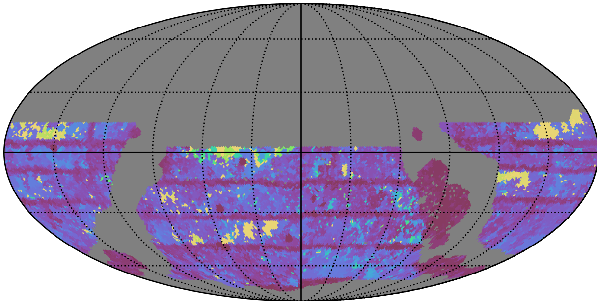
weather_cloudso1v3.4_10yrs WFD r band: Max Inter-Night Gap
