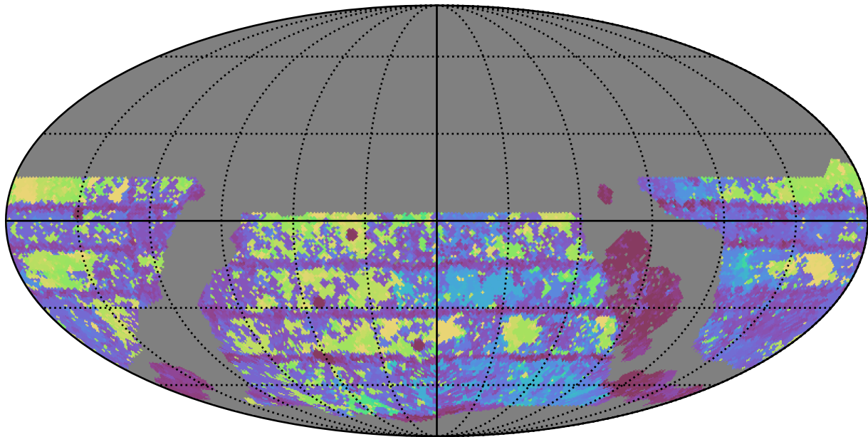
weather_cloudso1v3.4_10yrs WFD g band: Max Inter-Night Gap
