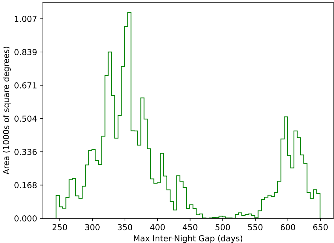
weather_cloudso1v3.4_10yrs WFD g band: Max Inter-Night Gap
