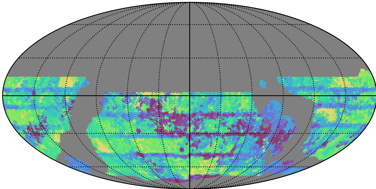
weather_cloudso1v3.4_10yrs WFD all bands: Max Inter-Night Gap
