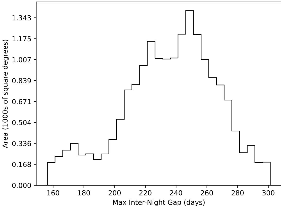
weather_cloudso1v3.4_10yrs WFD all bands: Max Inter-Night Gap
