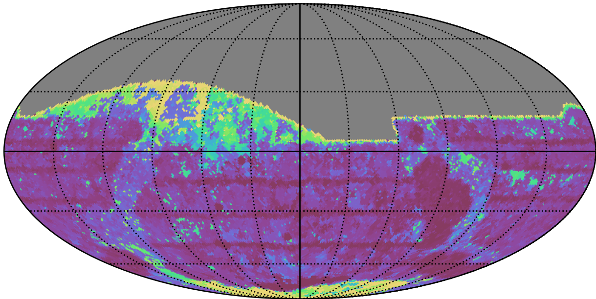
weather_cloudso1v3.4_10yrs All sky z band: Max Inter-Night Gap
