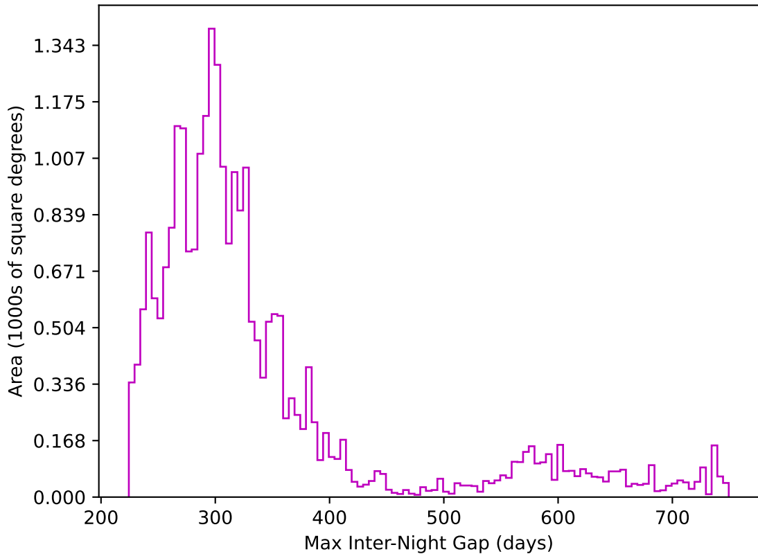
weather_cloudso1v3.4_10yrs All sky z band: Max Inter-Night Gap
