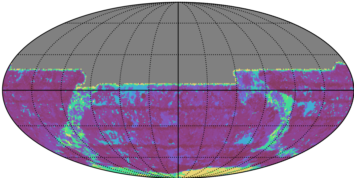
weather_cloudso1v3.4_10yrs All sky y band: Max Inter-Night Gap
